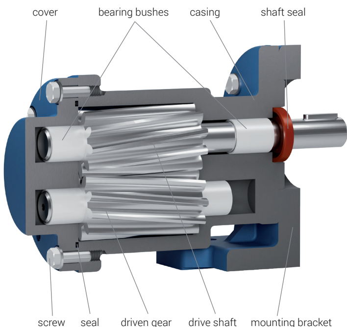
sectional drawing
