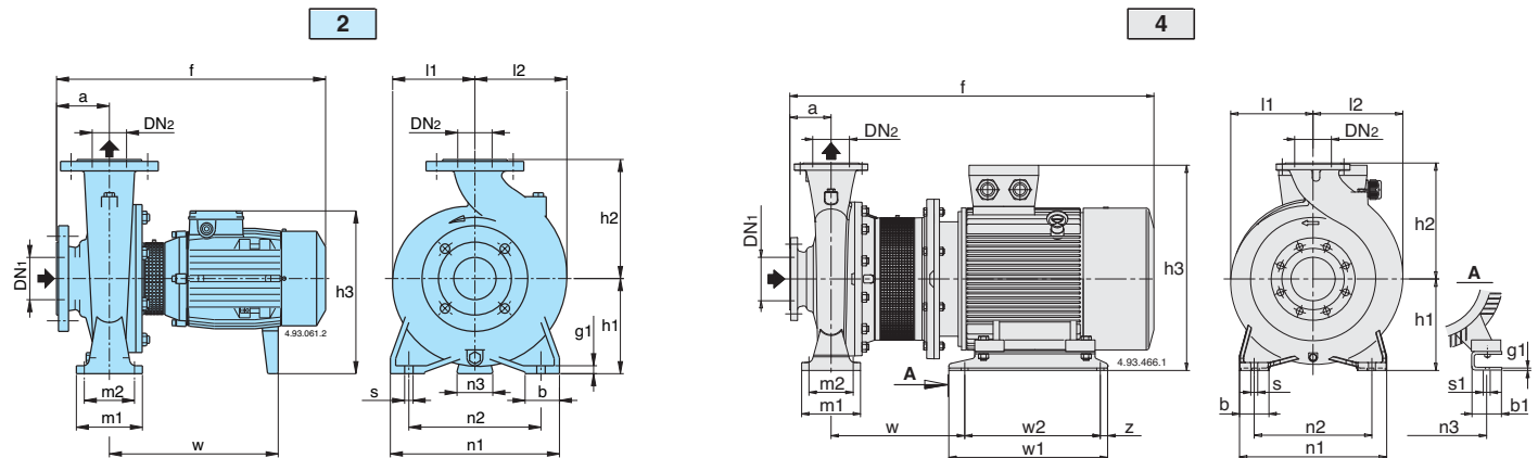
Standard construction
