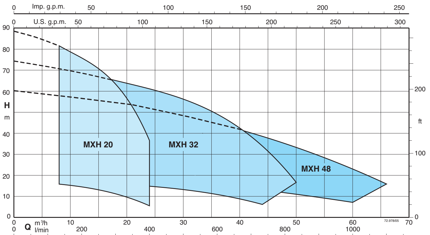
Coverage chart n \approx 2900 rpm
